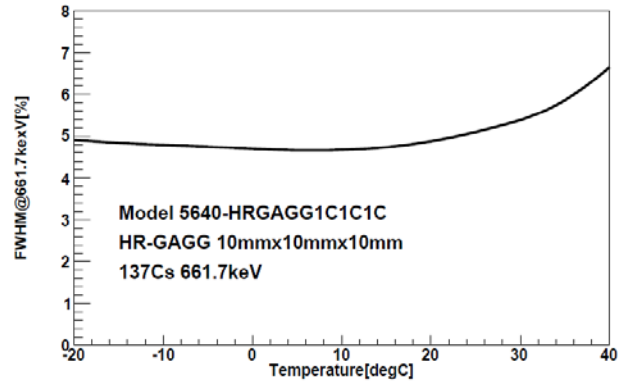
<Energy Resolution VS Temperature>
